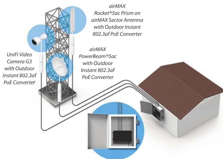
Outdoor Products Powered by 802.3af Switch
